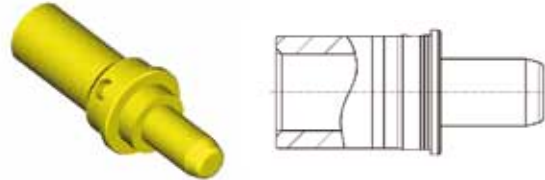
Pin contact
